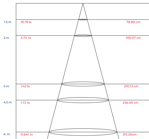
Lux-Distance Curve
